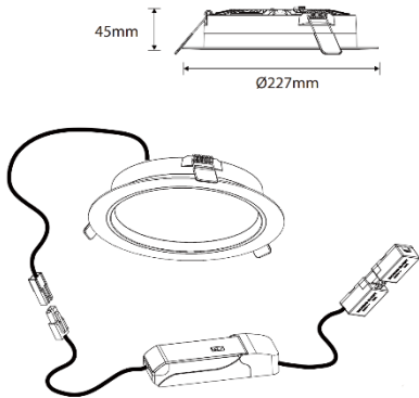
Dimension Diagram
